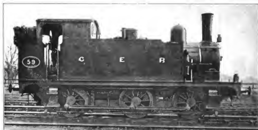
Fig. 5028. Six-Coupled Tank Shunting Locomotive. Great Eastern Railway. Cylinders 16 1/2 in. x 22 in.; Total Heating Surface 988.17 sq. ft.; Diameter of Drivers 48 in.; Weight on Drivers 95,100 lbs.; Total Weight 95,100 lbs.
